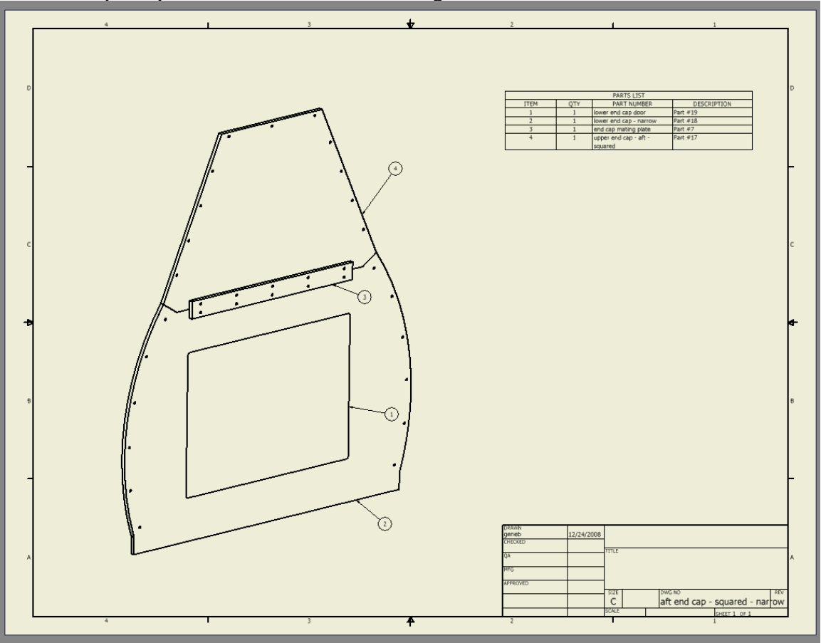
Aft End Cap – Squared – Narrow – Parts Arrangement
