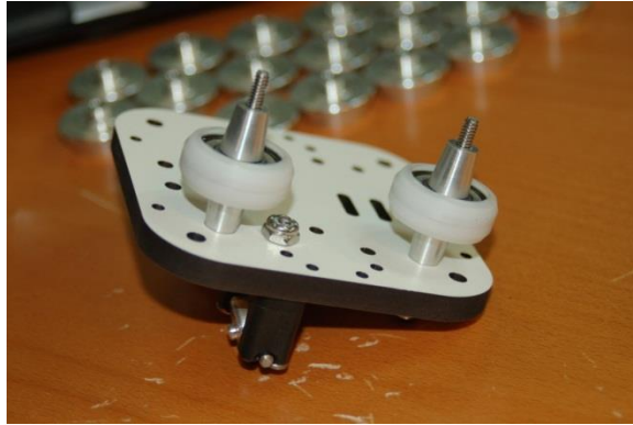
Figure 62 - Last Spacers Installed
